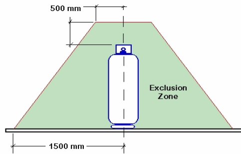
EXCHANGE CYLINDER HAZARDOUS ZONE Clearance to Ignition Sources
